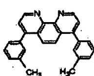
Structural formula 4:
